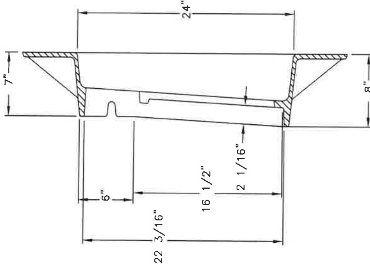
SECTION
