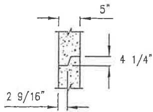
Joint Detail
