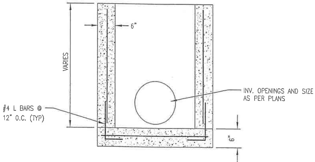
Section
