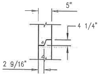
JOINT DETAIL
