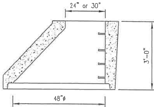
Eccentric Cone
